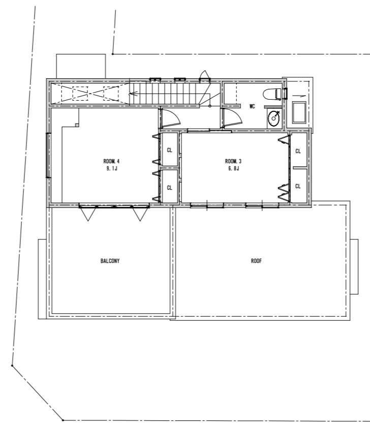
2F PLAN
